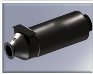
Combination Silencer and Diesel Oxidation Catalyst
