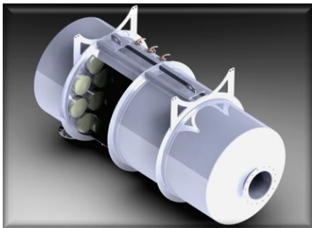
Integrated DPF / Silencer
